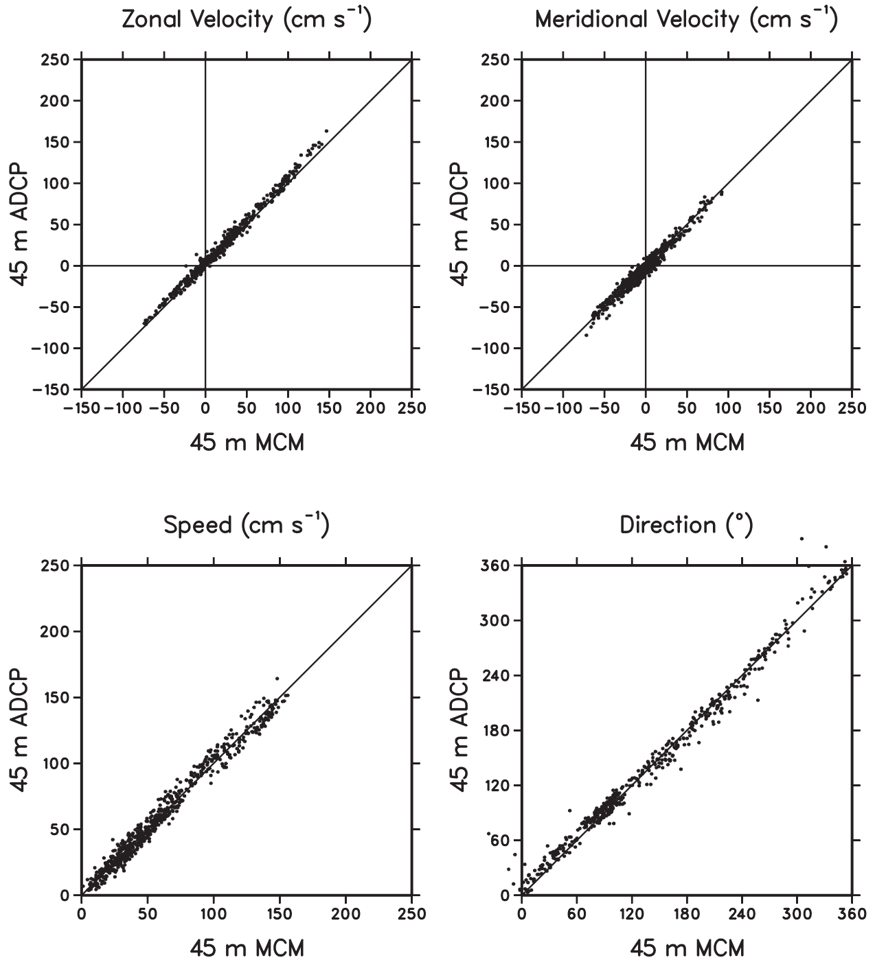
Figure 8: Scatter plot of 45 m daily averaged zonal velocity, meridional velocity, speed, and direction from MCMs and ADCPs measured from September 1996 to February 1999 at 0^{\circ}, 140^{\circ}\text{W} .
