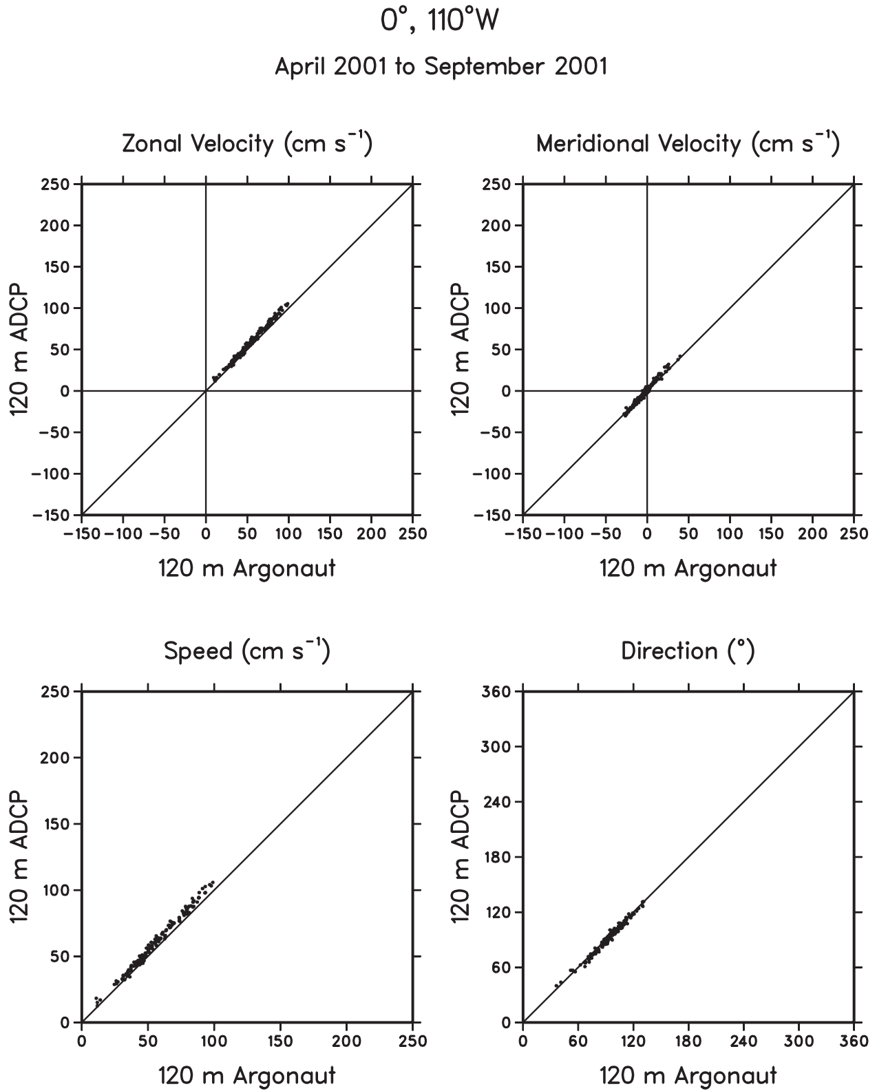
Figure 15: Scatter plot of 120 m daily averaged zonal velocity, meridional velocity, speed, and direction from Sontek Argonaut-MD current meters and ADCPs measured from April to September 2001 at 0^{\circ} , 110^{\circ} W.
